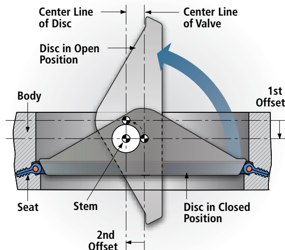
Disc in closed position; line pressure applied from the right.
