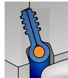
Seat non-compressed as disc approaches.
