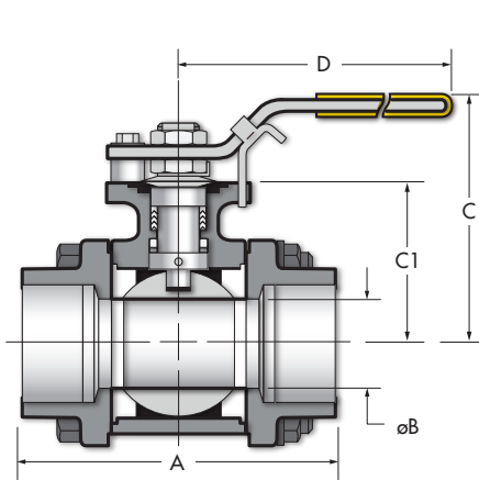
1/4" - 2 1/2" VALVES
