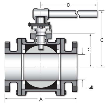
6" - 12" VALVES
