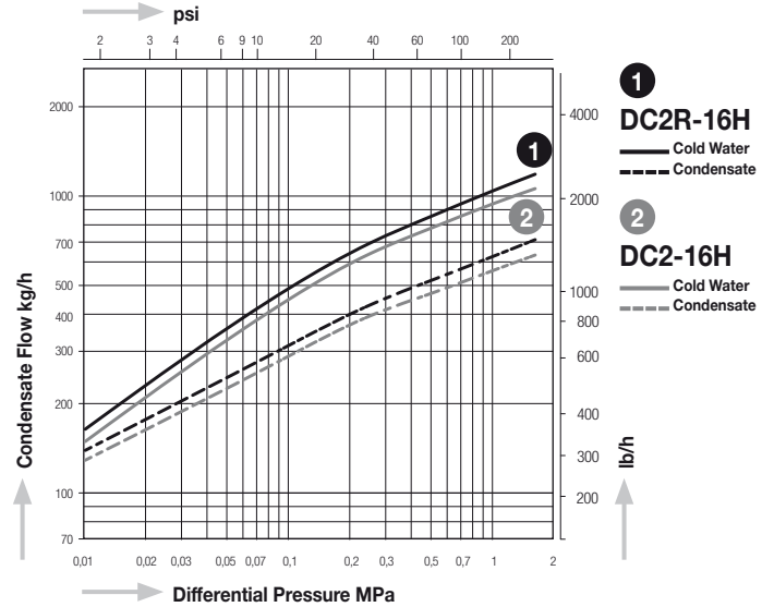
Capacity Chart
